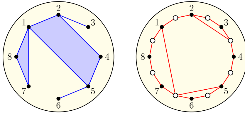
Figure 3: A noncrossing hypertree with 8 vertices and the corresponding even-sided dissection of a 16-gon.
